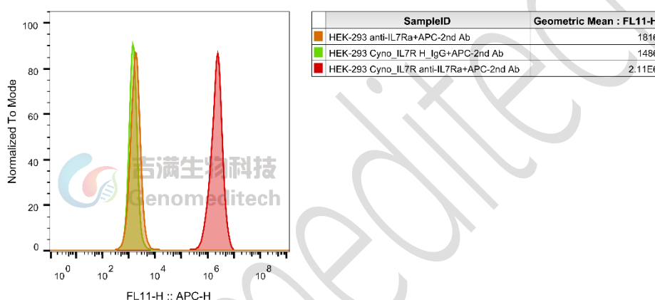
Figure 1 | Cynomolgus_IL7R HEK-293 Cell Line (Cat. GM-C39970) was determined by flow cytometry using Anti-IL7Ra hIgG1 Antibody(4A10) (Cat. GM-52274AB ).
